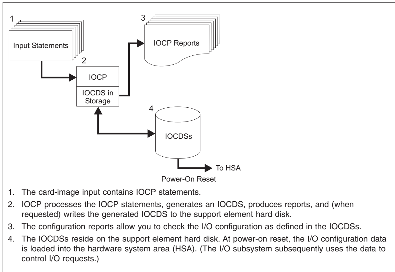
Figure 1-7. Overview of z/OS version of IOCP
