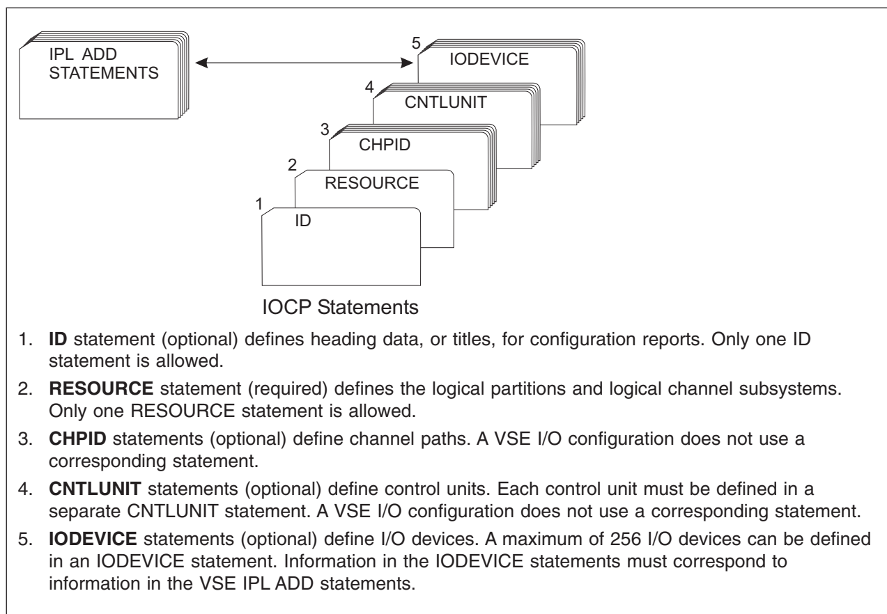
Figure 2-3. Correspondence between IOCP statements and VSE IPL ADD statements
