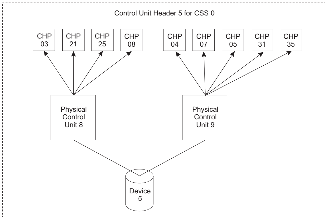
Figure 1-6. Control unit header that is incorrect
