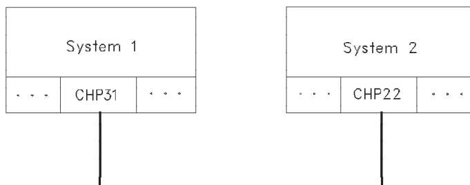
Figure E-3. ESCON CTC point-to-point
