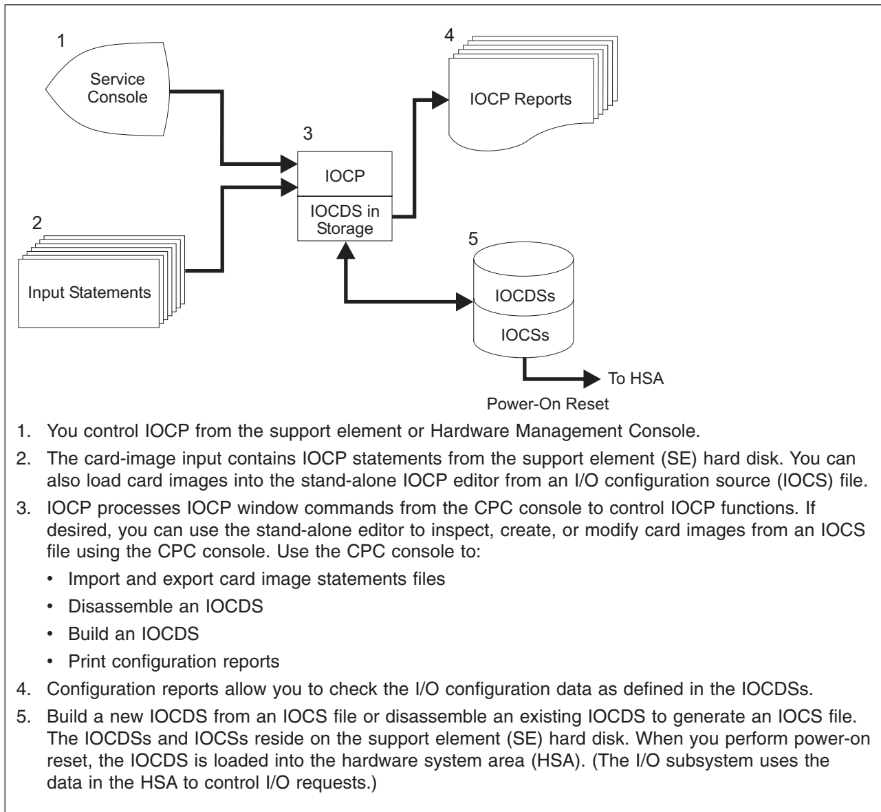
Figure 1-10. Overview of stand-alone version of IOCP
