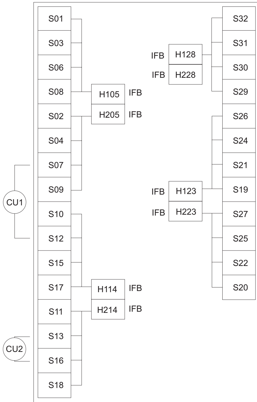
Figure 1-3. I/O channel path configuration for a representative I/O cage in a 2097 model
